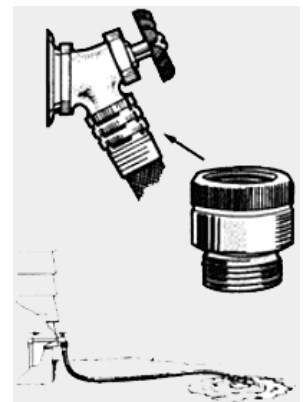
hose bib vacuum breaker
